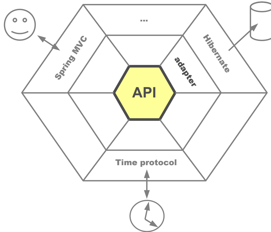
Ports and adapters pattern
